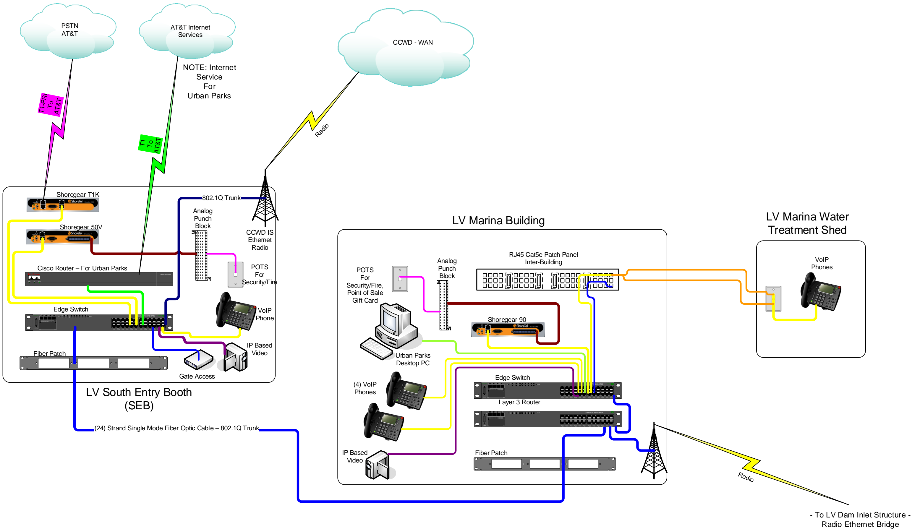
LV Marina Shoretel Phone / Data Diagram- March 30,2017
